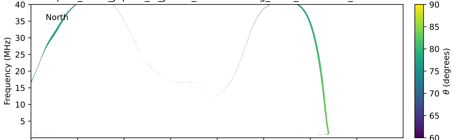
expres_earth_jupiter_io_jrm33_lossc-wid1deg_3kev_20230819_v11.cdf
