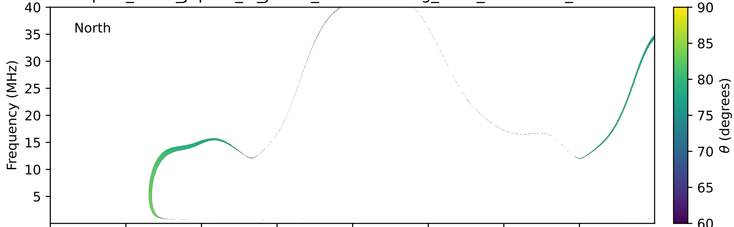
expres_earth_jupiter_io_jrm33_lossc-wid1deg_3kev_20230817_v11.cdf
