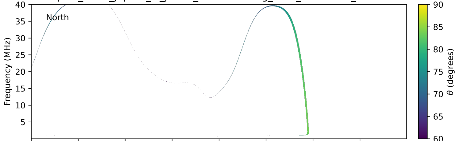
expres_earth_jupiter_io_jrm33_lossc-wid1deg_3kev_20230812_v11.cdf
