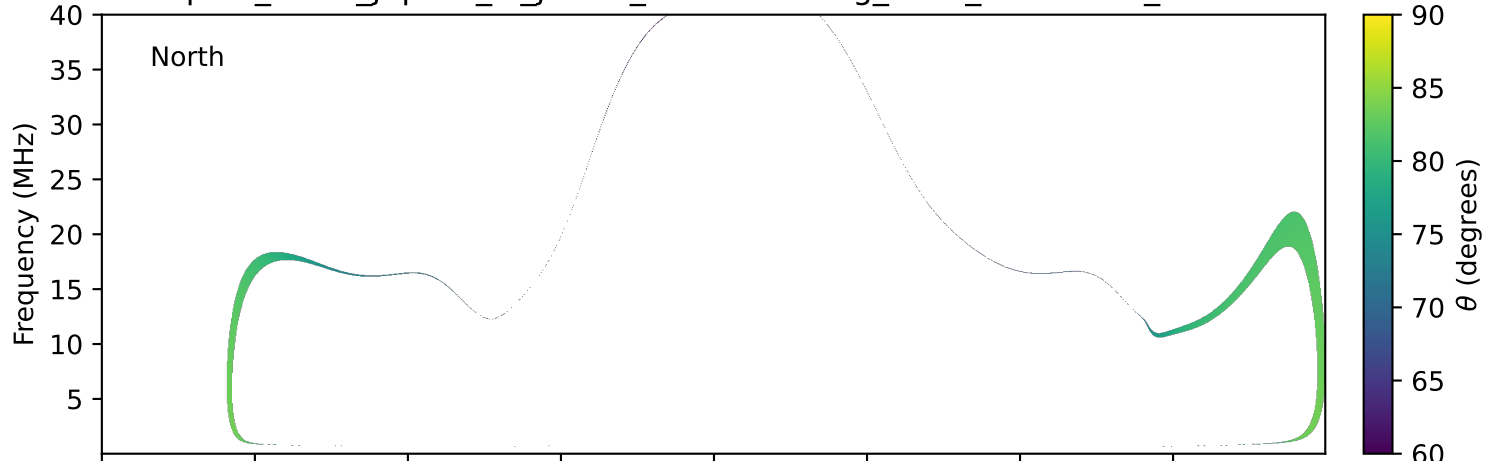
expres_earth_jupiter_io_jrm33_lossc-wid1deg_3kev_20230810_v11.cdf
