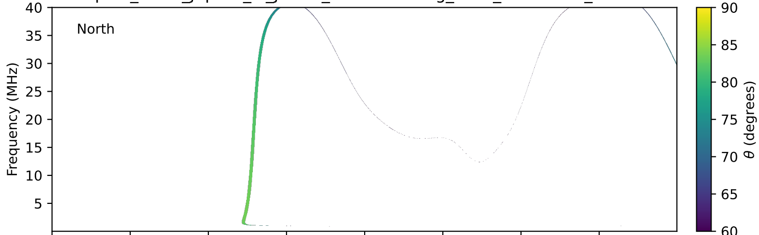
expres_earth_jupiter_io_jrm33_lossc-wid1deg_3kev_20230801_v11.cdf
