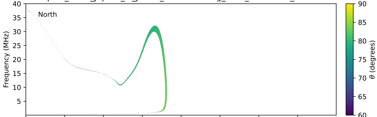
expres_earth_jupiter_io_jrm09_lossc-wid1deg_3kev_20230830_v11.cdf
