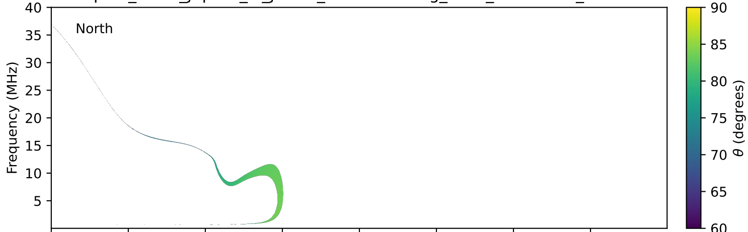
expres_earth_jupiter_io_jrm09_lossc-wid1deg_3kev_20230823_v11.cdf
