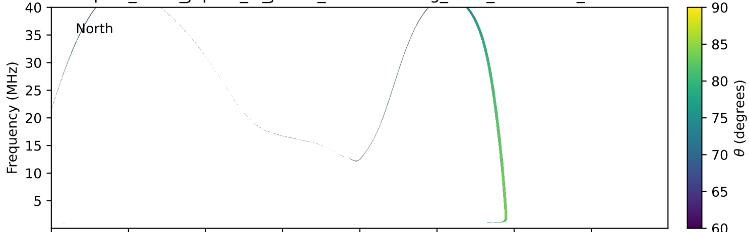
expres_earth_jupiter_io_jrm09_lossc-wid1deg_3kev_20230812_v11.cdf
