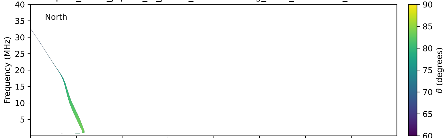
expres_earth_jupiter_io_jrm09_lossc-wid1deg_3kev_20230809_v11.cdf
