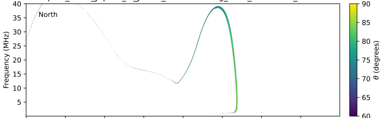
expres_earth_jupiter_io_jrm09_lossc-wid1deg_3kev_20230805_v11.cdf
