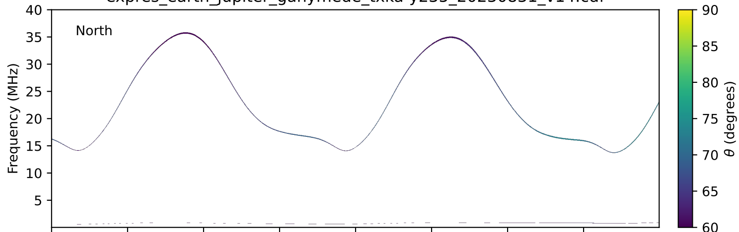
expres_earth_jupiter_ganymede_txka-y235_20230831_v14.cdf
