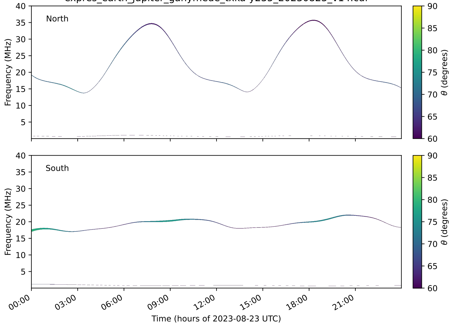
expres_earth_jupiter_ganymede_txka-y235_20230823_v14.cdf
