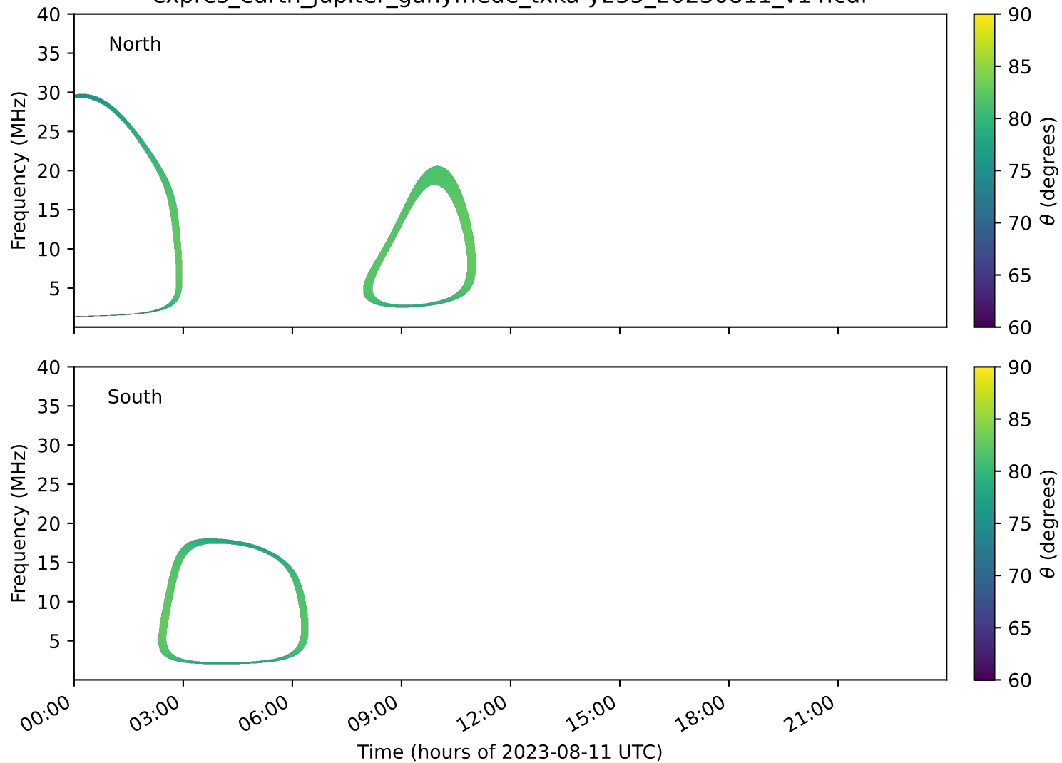
expres_earth_jupiter_ganymede_txka-y235_20230811_v14.cdf
