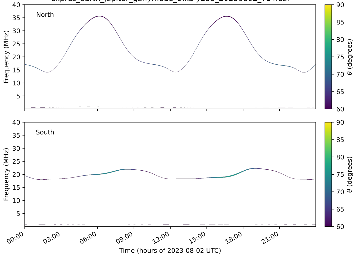
expres_earth_jupiter_ganymede_txka-y235_20230802_v14.cdf
