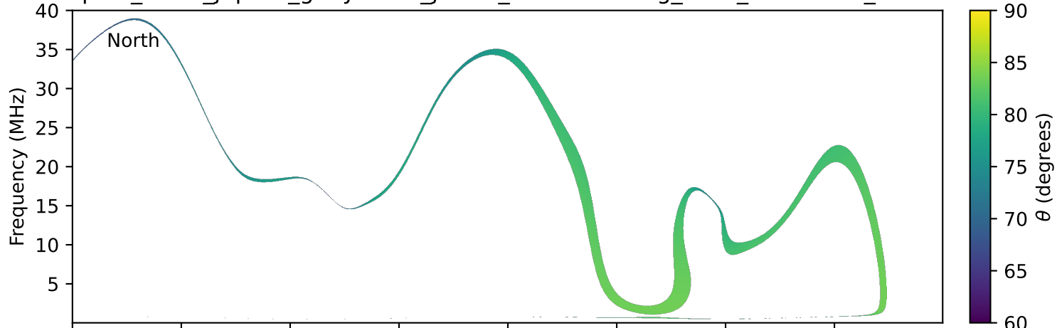
expres_earth_jupiter_ganymede_jrm33_lossc-wid1deg_3kev_20230825_v11.cdf
