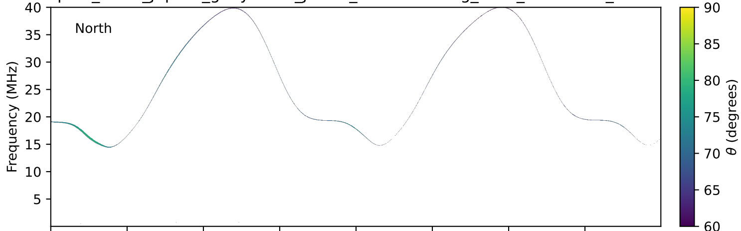
expres_earth_jupiter_ganymede_jrm33_lossc-wid1deg_3kev_20230816_v11.cdf
