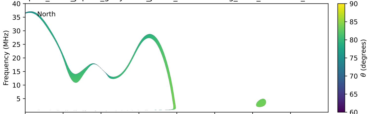
expres_earth_jupiter_ganymede_jrm33_lossc-wid1deg_3kev_20230811_v11.cdf
