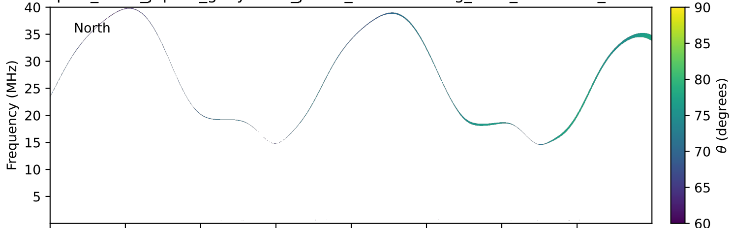
expres_earth_jupiter_ganymede_jrm33_lossc-wid1deg_3kev_20230803_v11.cdf
