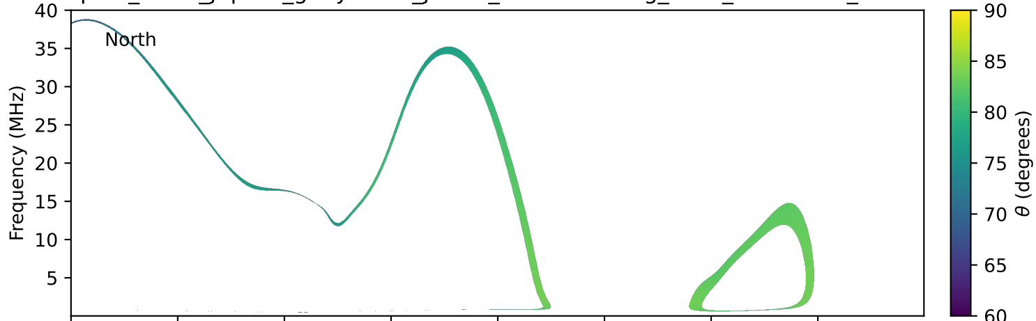
expres_earth_jupiter_ganymede_jrm09_lossc-wid1deg_3kev_20230818_v11.cdf
