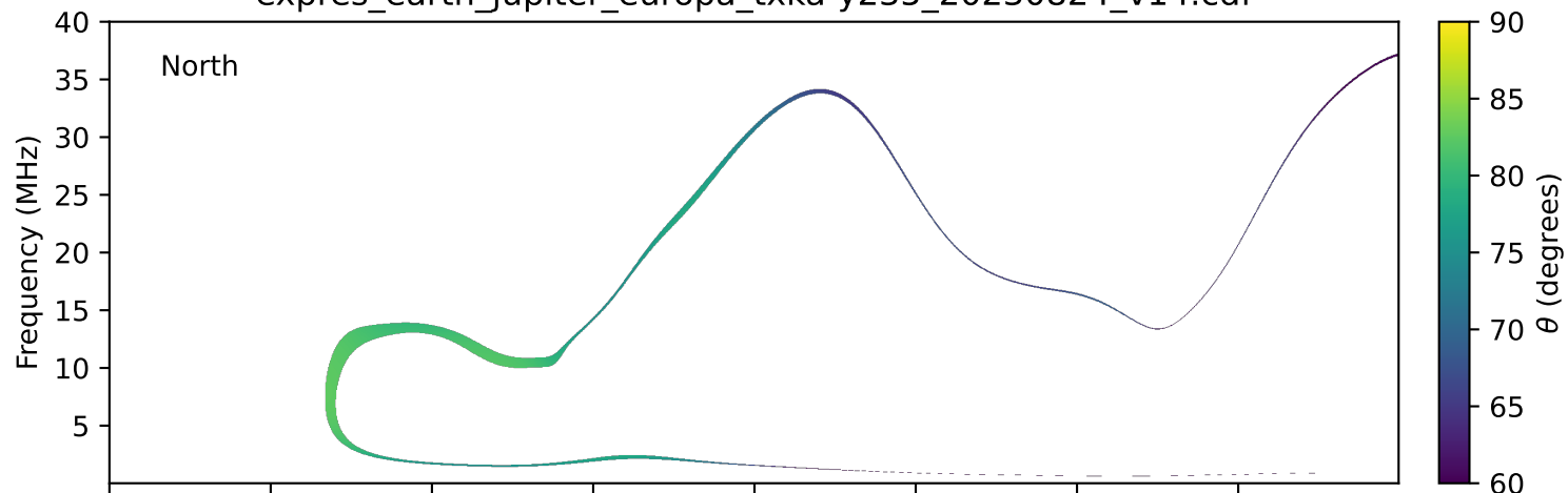
expres_earth_jupiter_europa_txka-y235_20230824_v14.cdf
