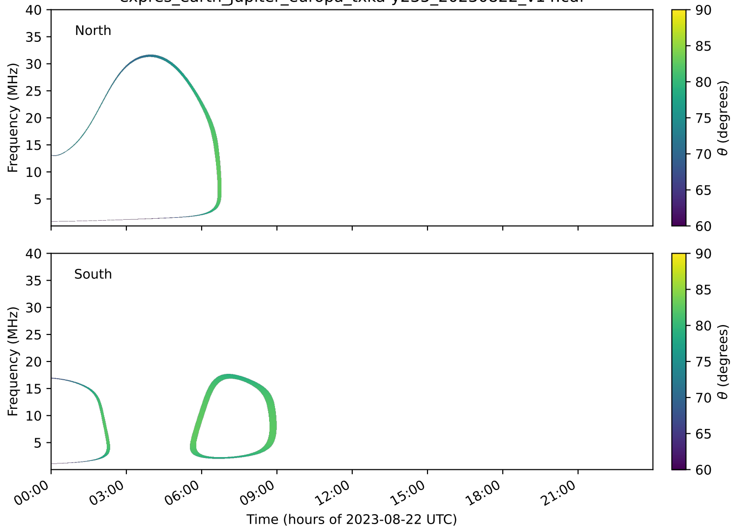
expres_earth_jupiter_europa_txka-y235_20230822_v14.cdf
