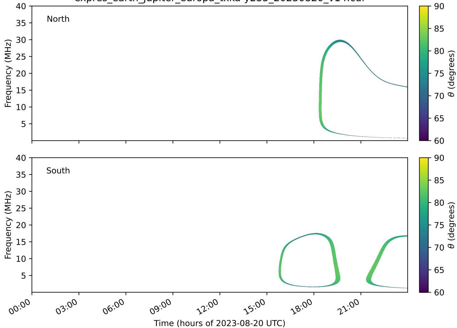
expres_earth_jupiter_europa_txka-y235_20230820_v14.cdf
