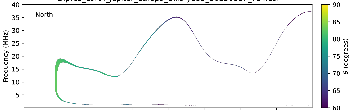
expres_earth_jupiter_europa_txka-y235_20230817_v14.cdf
