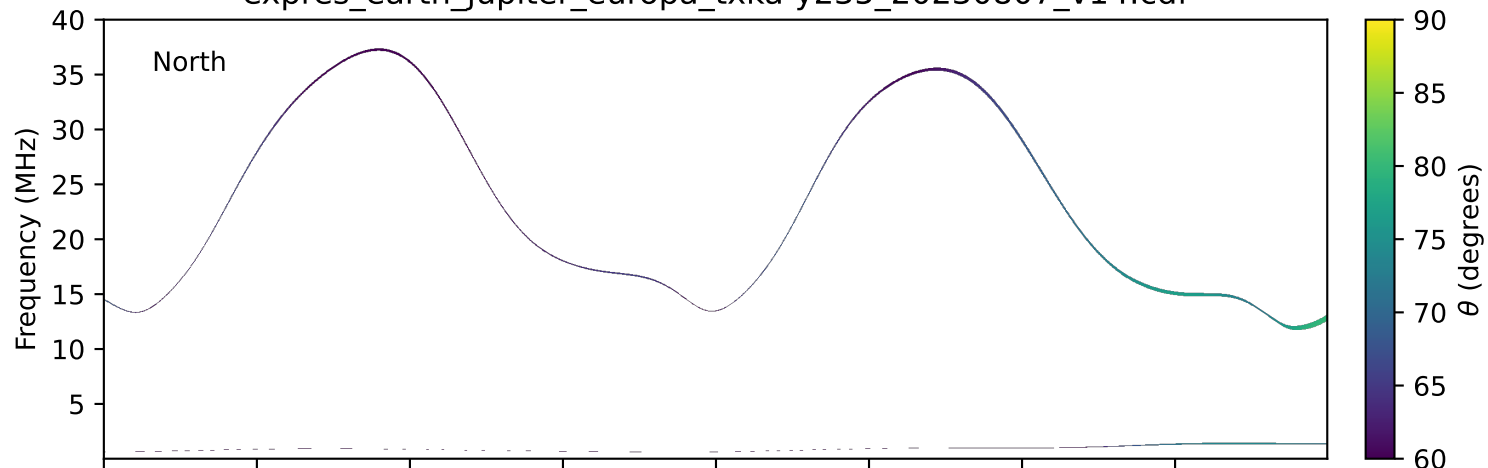
expres_earth_jupiter_europa_txka-y235_20230807_v14.cdf
