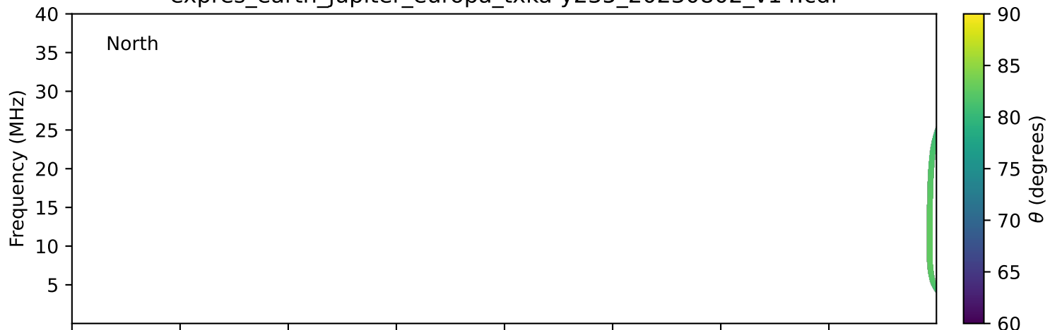
expres_earth_jupiter_europa_txka-y235_20230802_v14.cdf
