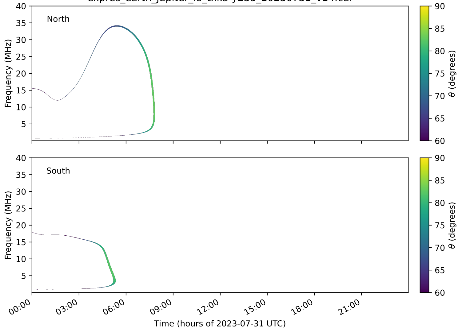
expres_earth_jupiter_io_txka-y235_20230731_v14.cdf
