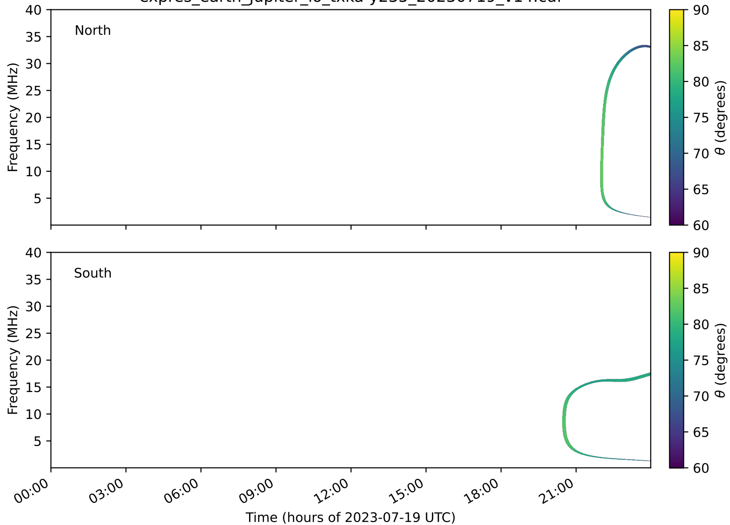
expres_earth_jupiter_io_txka-y235_20230719_v14.cdf
