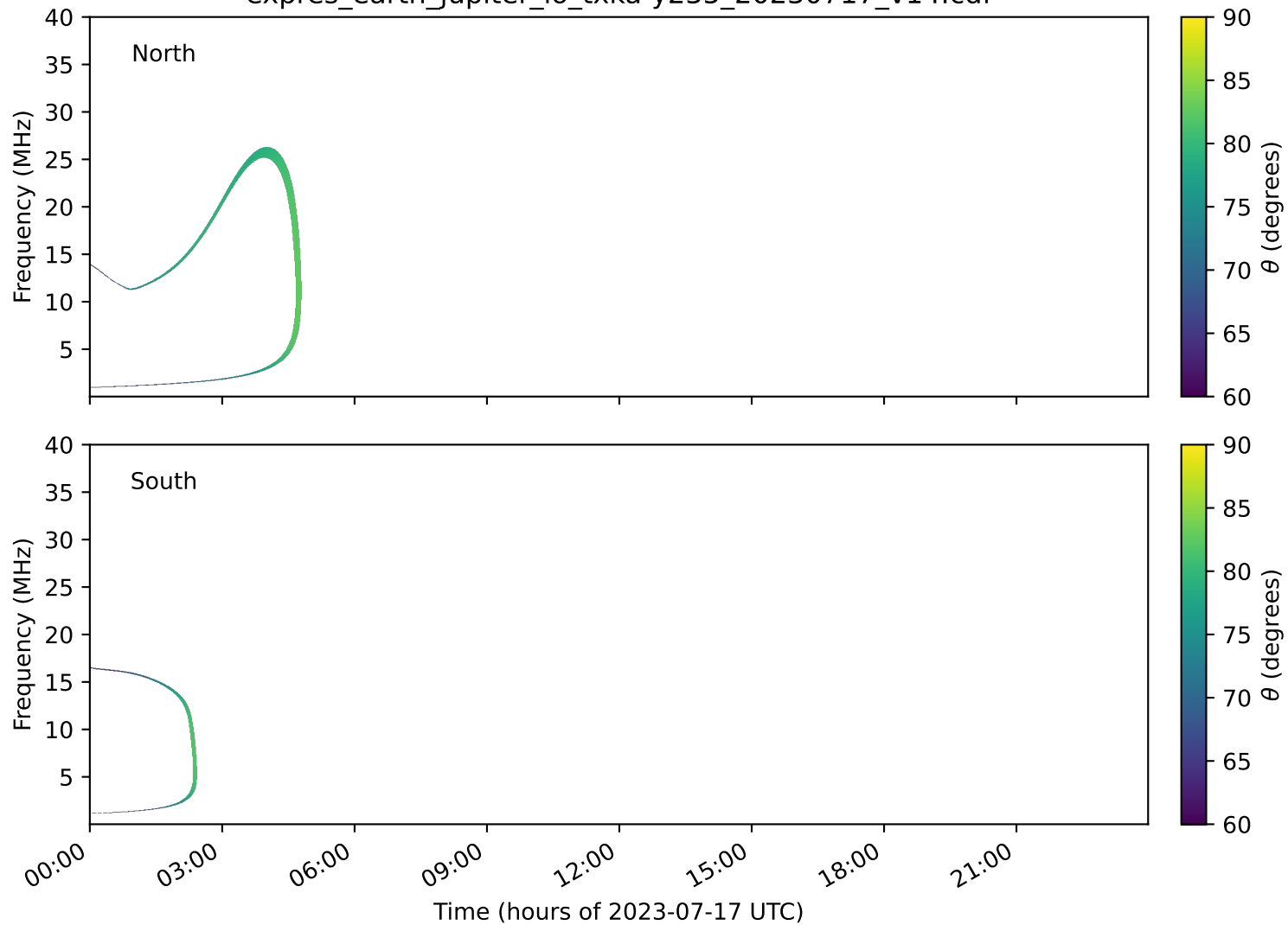
expres_earth_jupiter_io_txka-y235_20230717_v14.cdf
