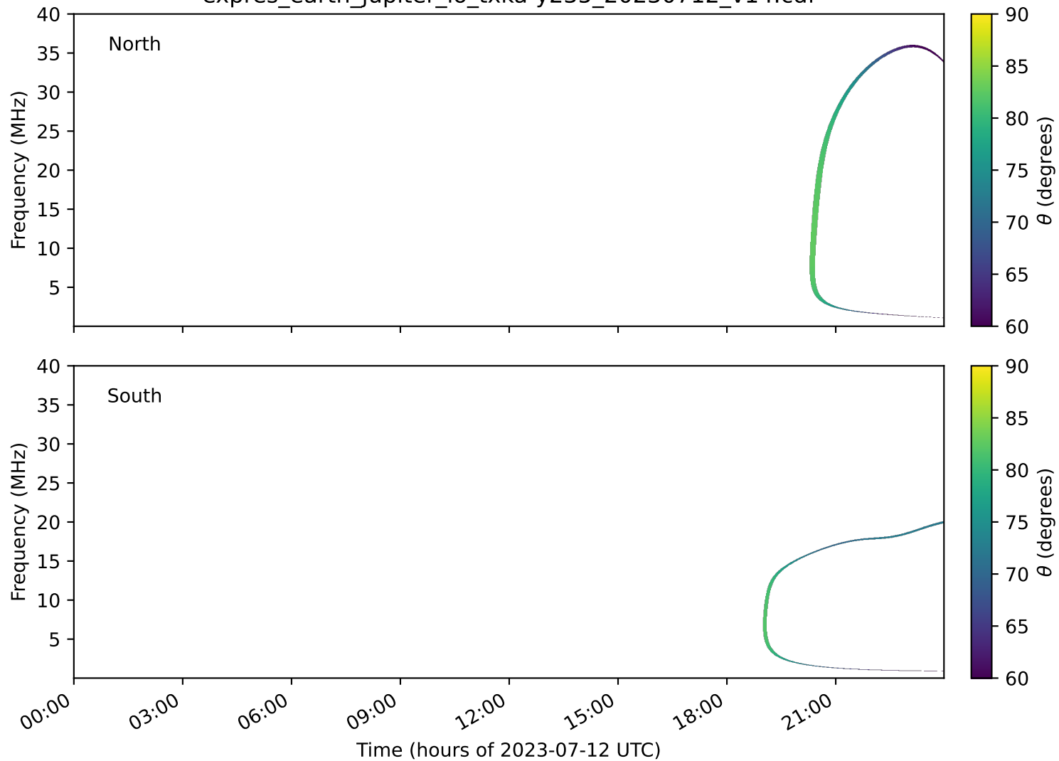
expres_earth_jupiter_io_txka-y235_20230712_v14.cdf
