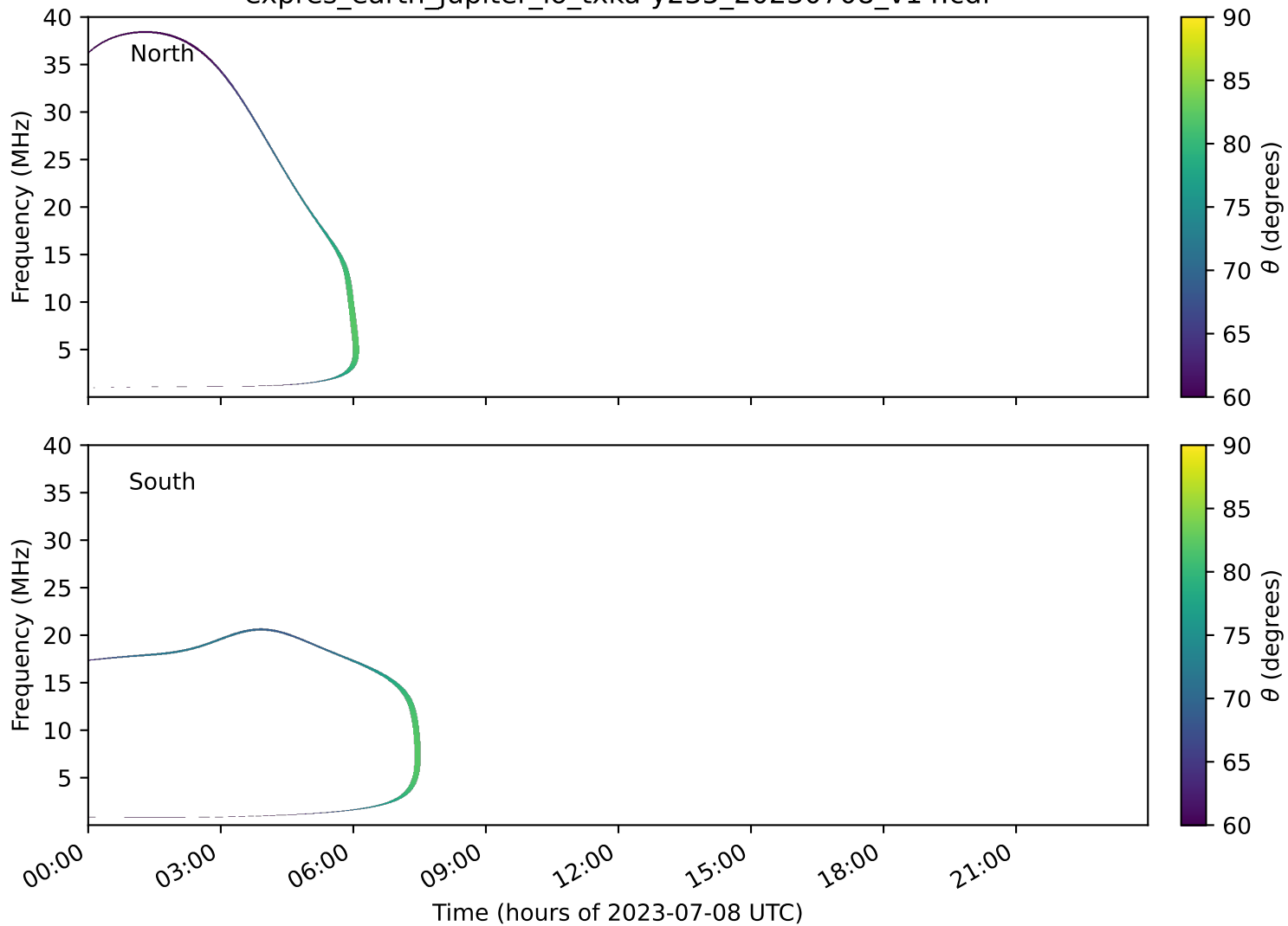
expres_earth_jupiter_io_txka-y235_20230708_v14.cdf
