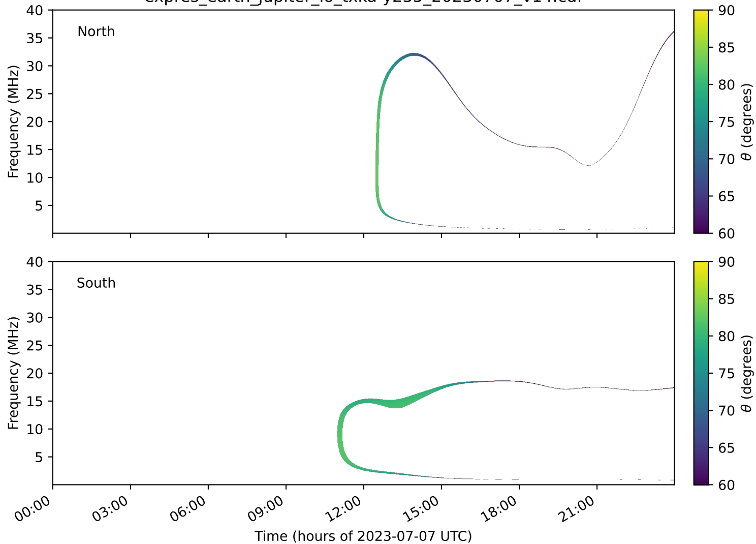
expres_earth_jupiter_io_txka-y235_20230707_v14.cdf
