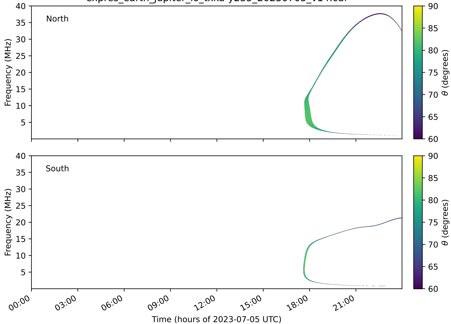
expres_earth_jupiter_io_txka-y235_20230705_v14.cdf
