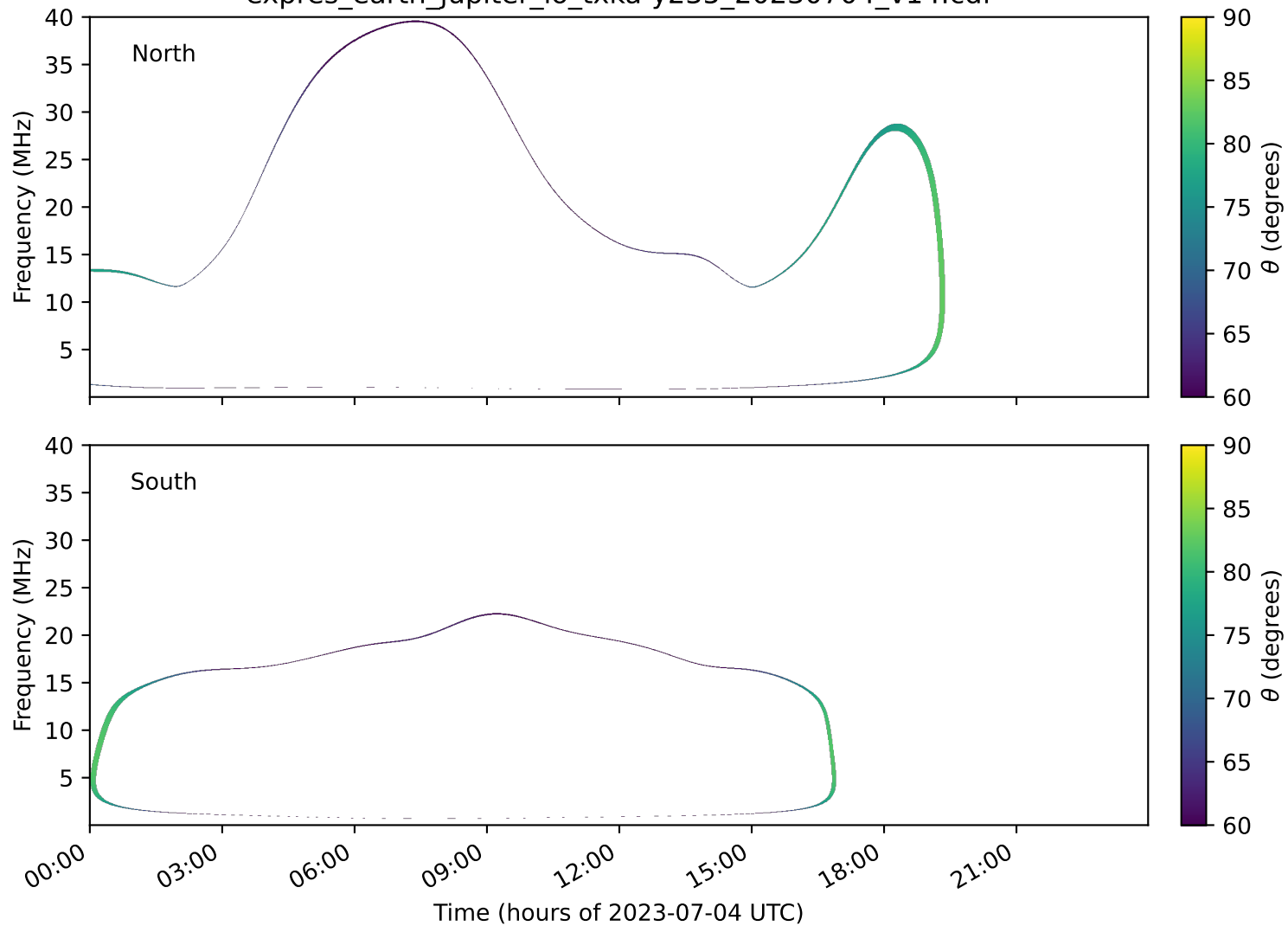
expres_earth_jupiter_io_txka-y235_20230704_v14.cdf
