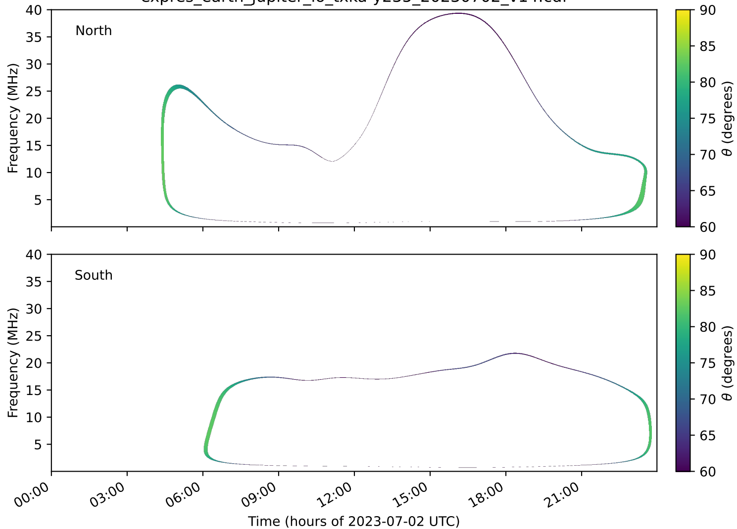
expres_earth_jupiter_io_txka-y235_20230702_v14.cdf
