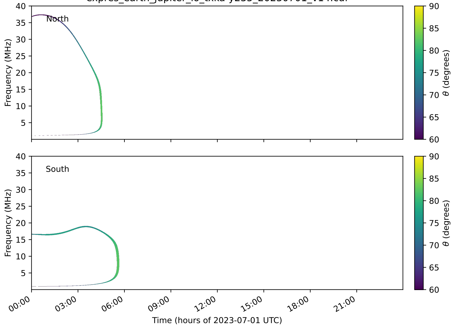
expres_earth_jupiter_io_txka-y235_20230701_v14.cdf
