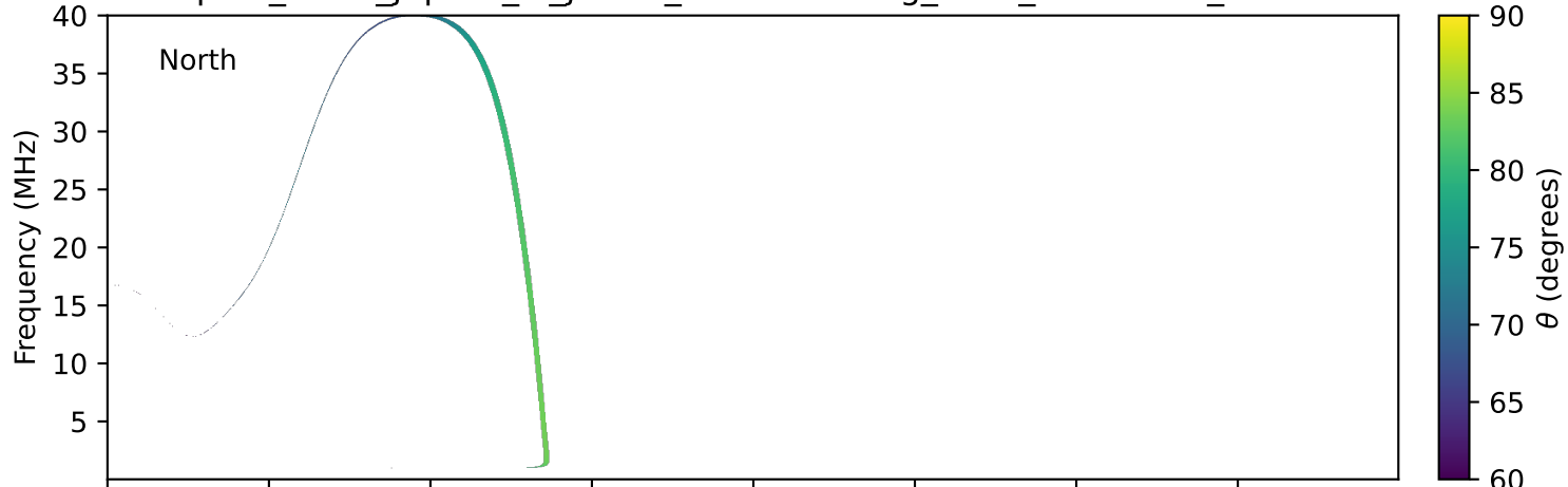
expres_earth_jupiter_io_jrm33_lossc-wid1deg_3kev_20230731_v11.cdf
