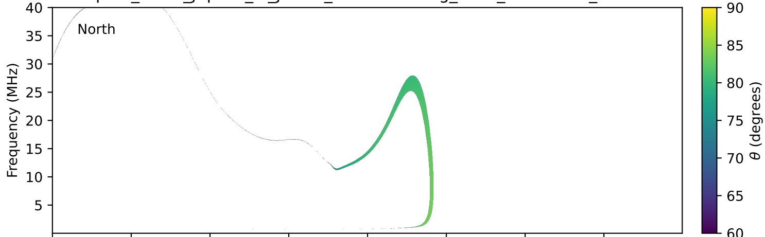
expres_earth_jupiter_io_jrm33_lossc-wid1deg_3kev_20230729_v11.cdf
