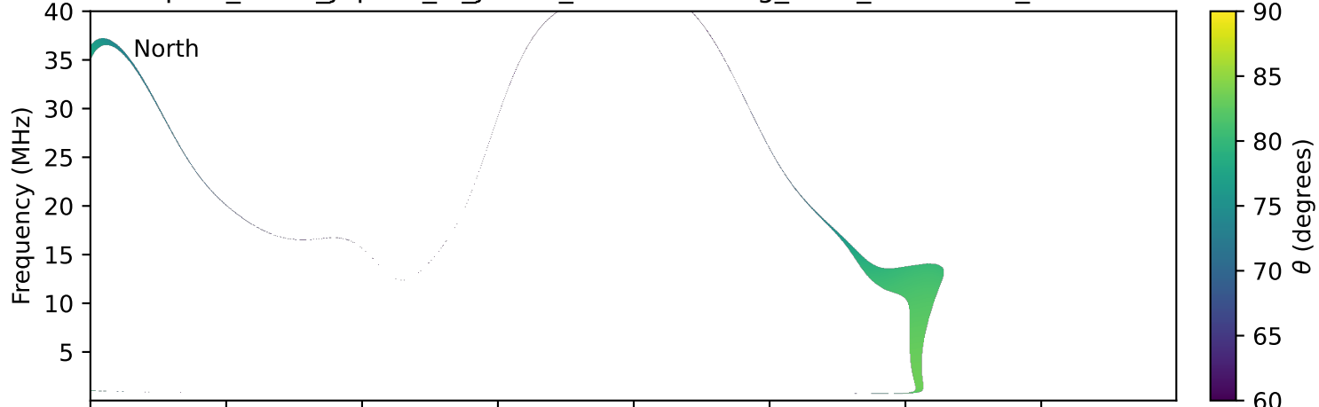
expres_earth_jupiter_io_jrm33_lossc-wid1deg_3kev_20230727_v11.cdf
