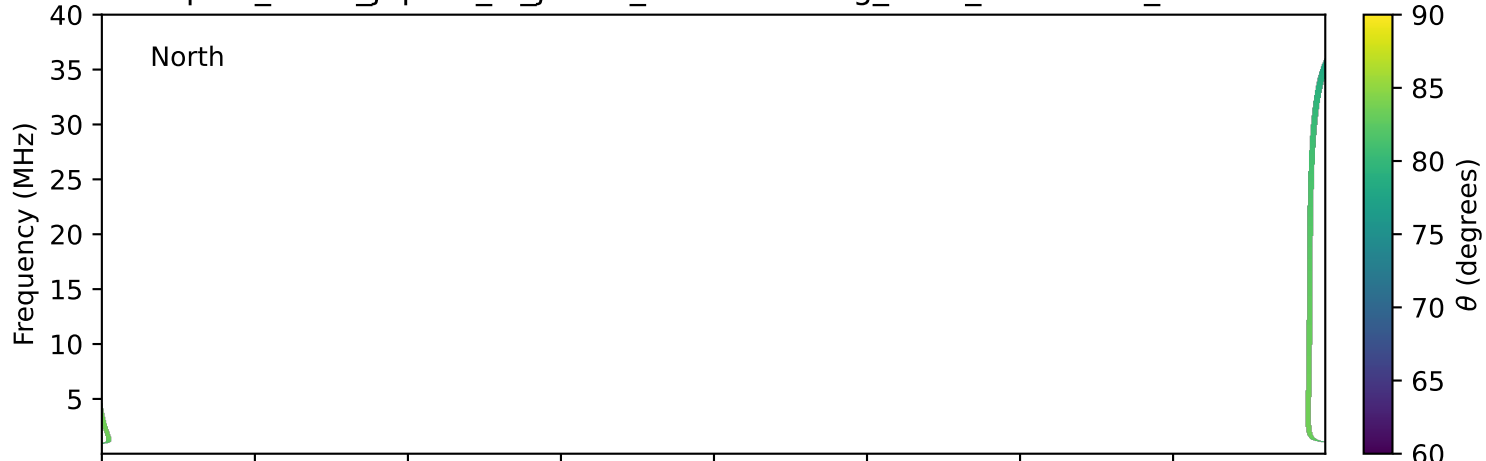
expres_earth_jupiter_io_jrm33_lossc-wid1deg_3kev_20230726_v11.cdf
