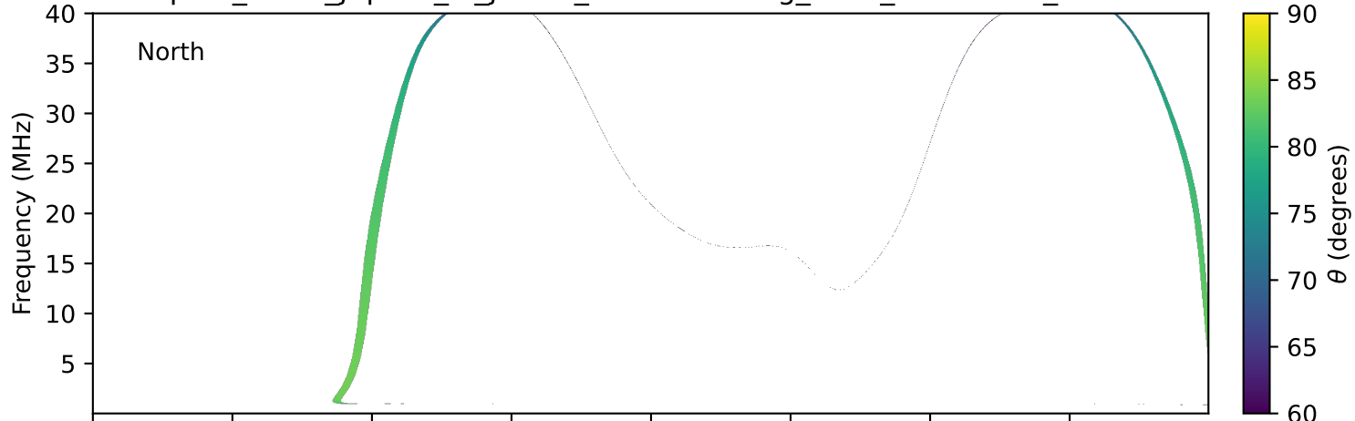
expres_earth_jupiter_io_jrm33_lossc-wid1deg_3kev_20230725_v11.cdf
