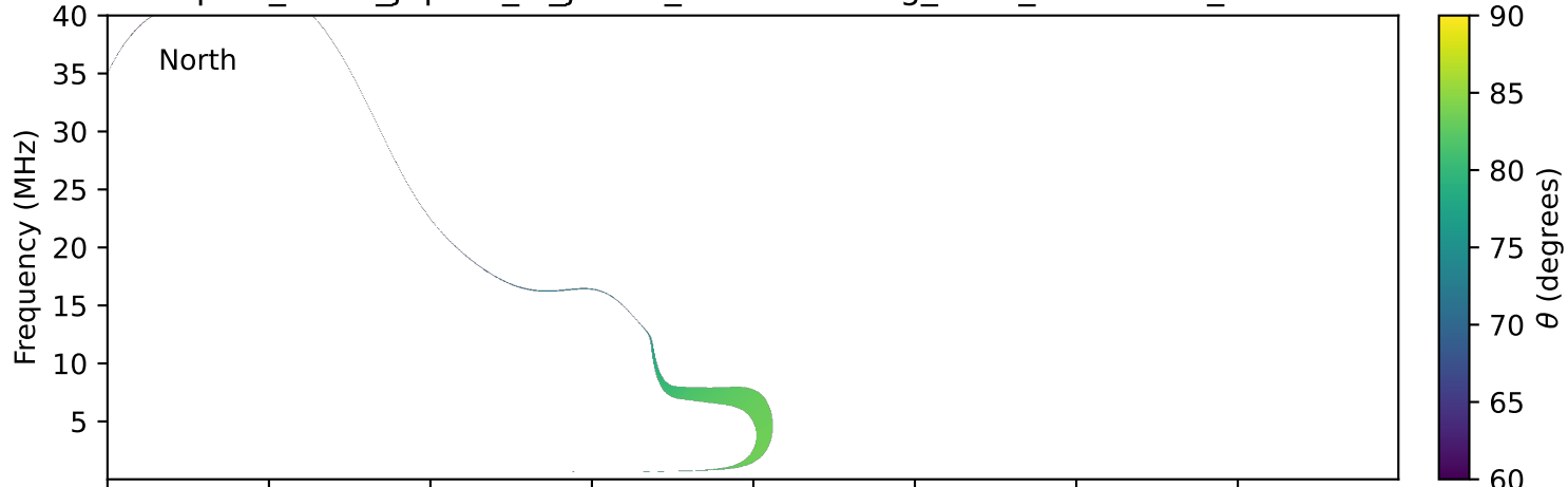
expres_earth_jupiter_io_jrm33_lossc-wid1deg_3kev_20230722_v11.cdf
