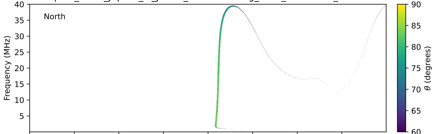
expres_earth_jupiter_io_jrm33_lossc-wid1deg_3kev_20230707_v11.cdf
