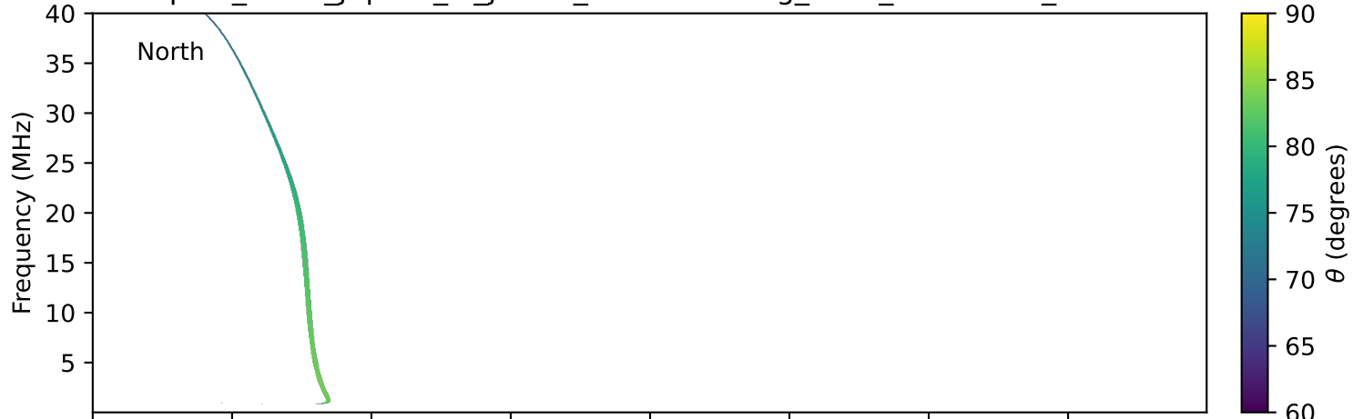
expres_earth_jupiter_io_jrm33_lossc-wid1deg_3kev_20230701_v11.cdf
