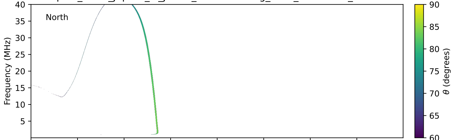
expres_earth_jupiter_io_jrm09_lossc-wid1deg_3kev_20230731_v11.cdf
