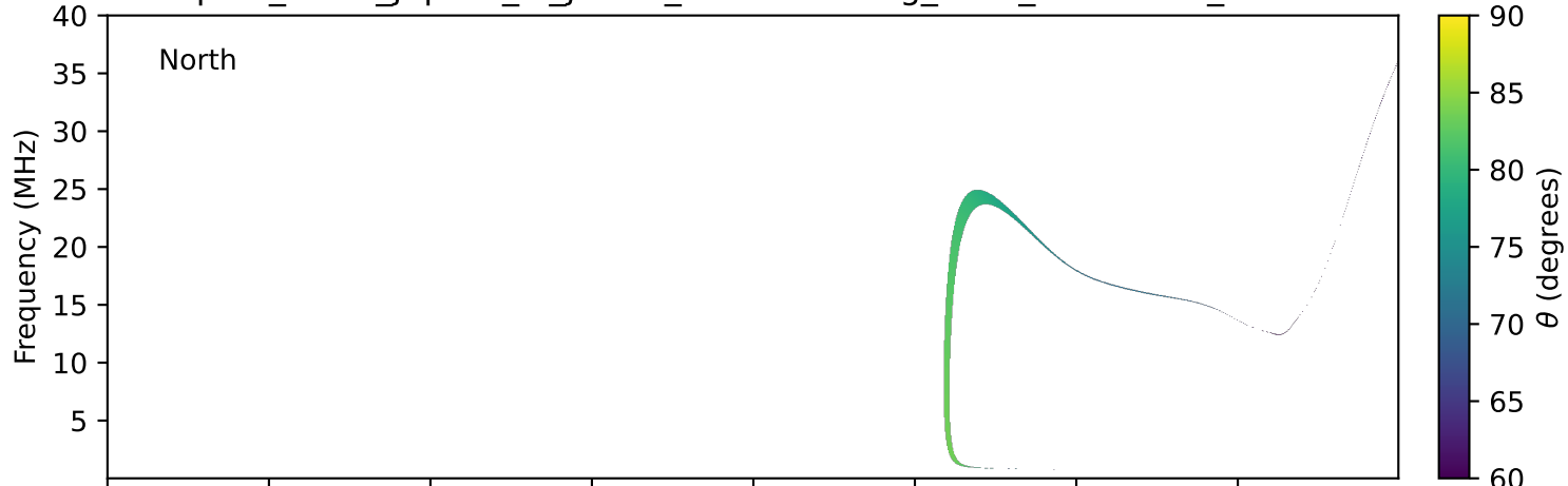
expres_earth_jupiter_io_jrm09_lossc-wid1deg_3kev_20230721_v11.cdf
