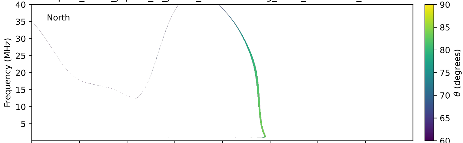
expres_earth_jupiter_io_jrm09_lossc-wid1deg_3kev_20230713_v11.cdf
