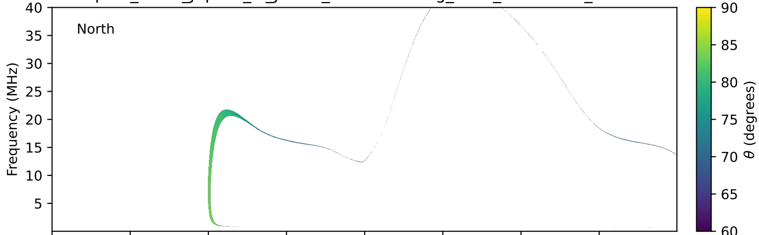
expres_earth_jupiter_io_jrm09_lossc-wid1deg_3kev_20230709_v11.cdf
