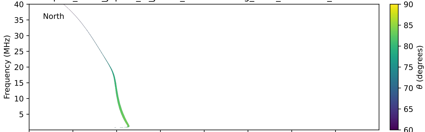
expres_earth_jupiter_io_jrm09_lossc-wid1deg_3kev_20230708_v11.cdf
