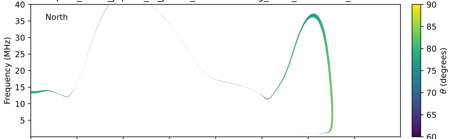
expres_earth_jupiter_io_jrm09_lossc-wid1deg_3kev_20230704_v11.cdf
