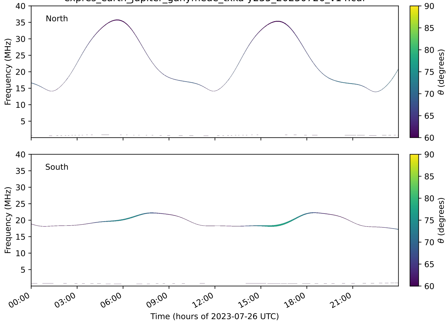
expres_earth_jupiter_ganymede_txka-y235_20230726_v14.cdf
